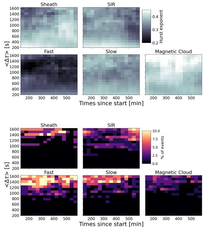
Figure 5. (Top) Colour maps showing the values of the local Hurst exponent as a function of time (given in minutes from the start of the solar wind time interval) and the mid-point of the time-lag interval used to calculate the Hurst exponent (see text for details). (Bottom) The percentage of the events for which the standard error related to the fitting was > 0.05 . These events were removed from the analysis.
