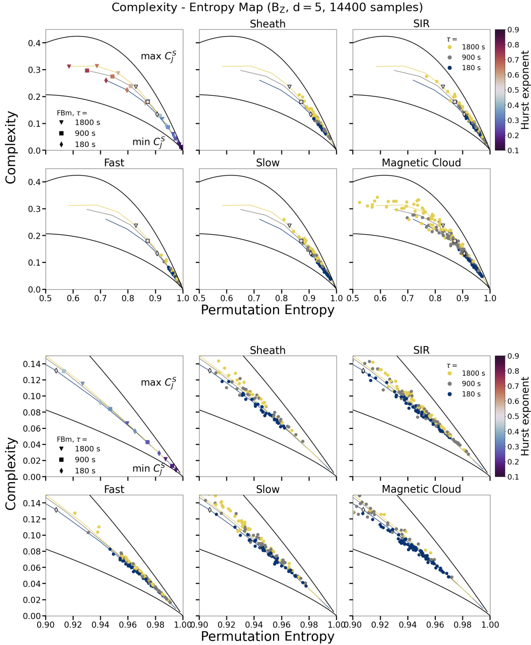
Figure 4. Complexity–entropy maps showing Jensen-Shannon complexity in B_Z plotted against normalized permutation entropy for d = 5 and sub-sampling rates ranging from r = 20 to 600 in steps of 60 ( \tau = 60 to 1800 s in steps of 60 s). The dark blue points show values for r = 20 , with point colour darkening to yellow with increasing r . In the top left panel the grey square and diamond markers show the fractional Brownian motion calculated with r = 20 and r = 600 , respectively, for Hurst exponents from 0.1 to 0.8. The markers repeated in all panels with black edges indicate H = 0.5 . Minimum and maximum complexity curves are shown in black.
